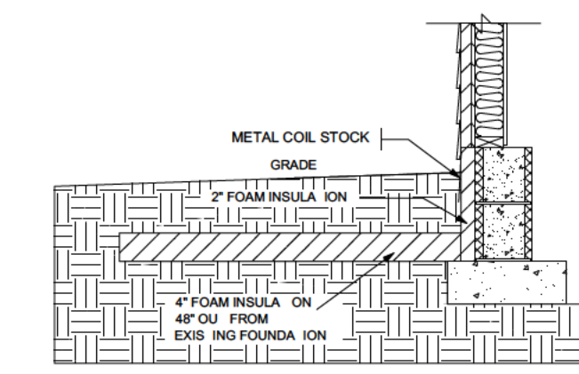
EXISTING HOUSE / FOUNDATION DETAIL
